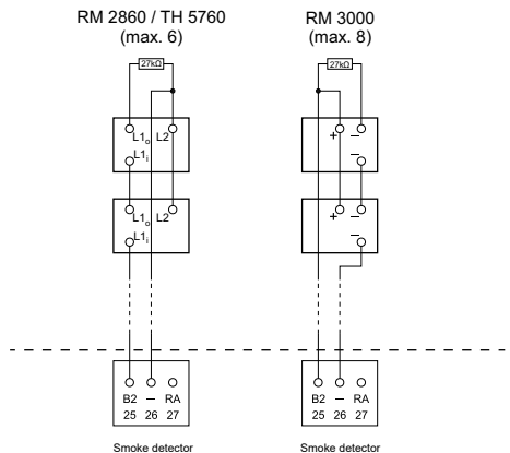
Figure 9: Wiring diagram smoke detector
