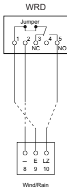
Figure 7: Wiring diagram wind / rain detector
