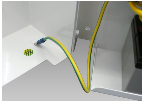
Figure 13: PE connection
