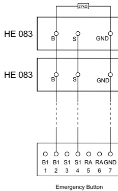
Figure 6: Wiring diagram emergency button HE 083
