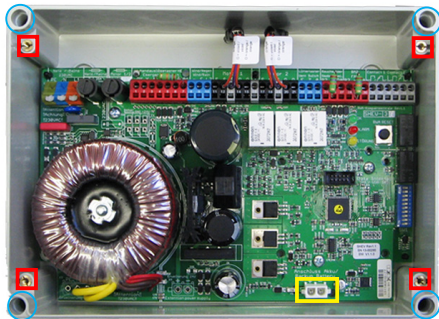
Figure 2: Mounting points SP 300 plastic housing (SP 600 analog)
