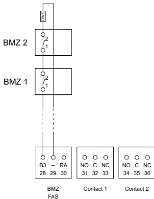
Figure 11: Wiring diagram contact FAS
