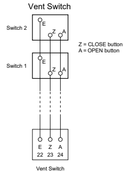
Figure 8: Wiring diagram ventilation button
