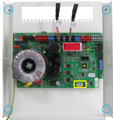
Figure 4: Mounting points SP 300-IP (SP 600 analog)
