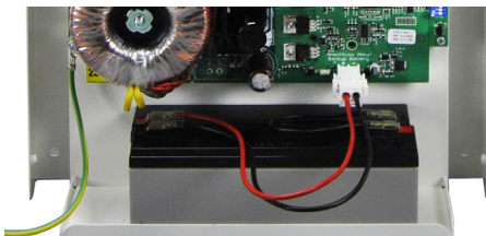
Figure 12: Battery connection SP 300-AP steel sheet housing (SP 600 analog)
