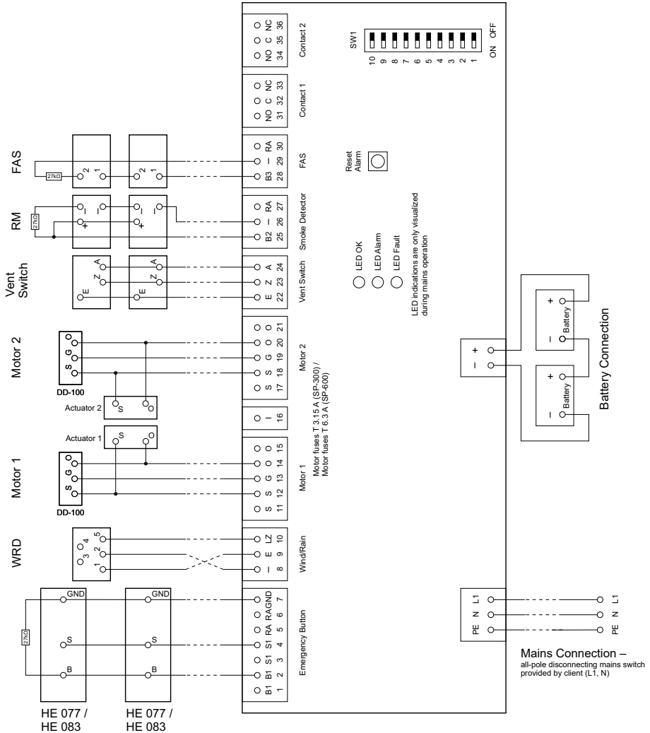
Figure 5: Wiring diagram complete (simplified illustration)
